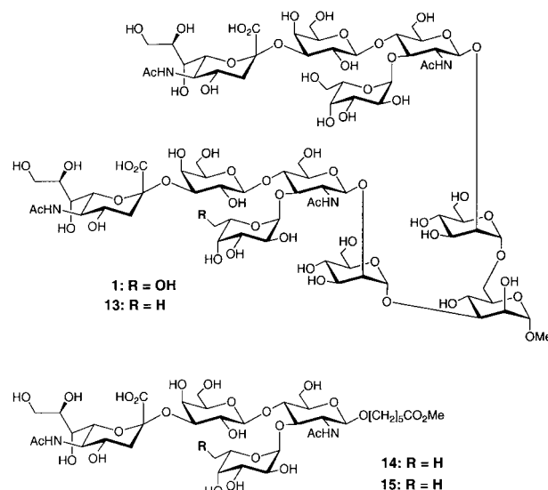
Figure 3. Monomeric and dimeric SLe x analogues undergoing inhibition assays.
