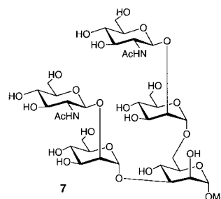
Figure 2. Pentasaccharide precursor for enzymatic decoration.
