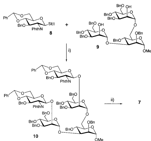
Scheme 2. (i) NIS, AgOTf, 4 Å ms, CH 2 Cl 2 , toluene, –50 °C to rt, 85%; (ii) (a) NH 2 NH 2 , EtOH; (b) Ac 2 O, pyridine; (c) K 2 CO 3 , MeOH; (d) Pd/C, CH 2 Cl 2 :EtOH:H 2 O 3:3:1, 79% over four steps.
