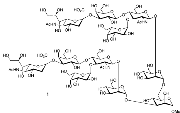
Figure 1. L-Galactosylated SLe x undecasaccharide.
