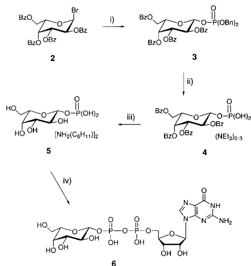
Scheme 1. (i) Ag 2 CO 3 , (Bn) 2 P(O)OH, CH 2 Cl 2 , Et 2 O, CH 3 CN, 93% over two steps; (ii) Pd/C, H 2 , toluene, pyridine, NEt 3 , 97%; (iii) MeOH, cyclohexylamine, 90%; (iv) BioRad AG 50W-X2 (NEt 3 -form), quant, then guanosinemorpholidate, tetrazole, pyridine, 3 days, 74%.
