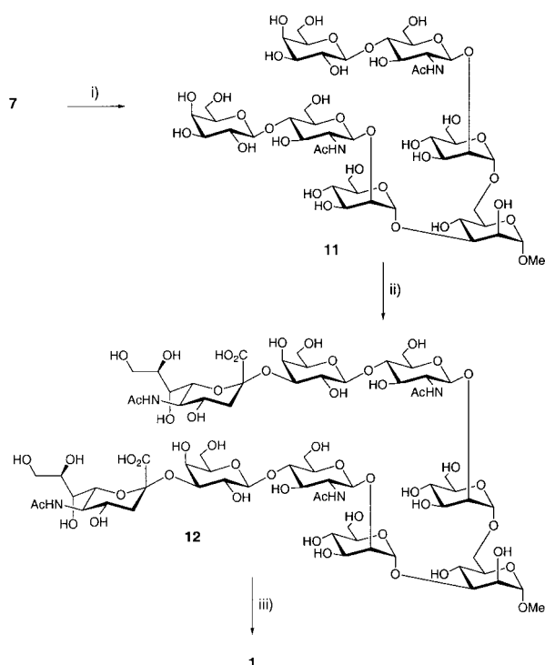
Scheme 3. (i) UDP-galactose, β-1,4-galactosyltransferase, alkaline phosphatase, BSA, HEPES (50 mM, pH 7.2), 69%; (ii) CMP-NeuAc, α-2,3-sialyltransferase, MnCl 2 , MgCl 2 , alkaline phosphatase, BSA, HEPES (200 mM, pH 7.5), 99%; (iii) GDP-L-galactose, α-1,3-fucosyltransferase V, MnCl 2 , alkaline phosphatase, BSA, MES (50 mM, pH 6.0), 56%.
